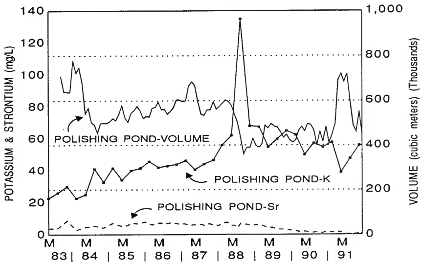
Figure 7.7 Lagoon Water Quality Data for Potassium, Strontium and Polishing Pond Volume, 1983 to 1991.
